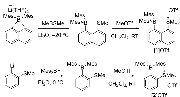
Scheme 1. Syntheses of [1] OTf and [2] OTf.
